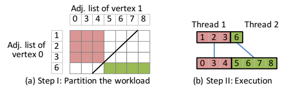
Fig. 4: Merge-based intersection.
