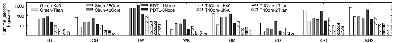
Fig. 10: The runtime of TRICORE and three related projects: Green [27] (on single K40c and single Titan X GPU), Shun [51] (on 28-core CPU and 48-core CPU) and PDDL [24] (on single node and 6 nodes of 16-core CPU). TRICORE-1K and TRICORE-6K are our results on one and six K40c GPUs respectively. Similarly, TRICORE-1Titan X and TRICORE-2Titan X are our results on one and two Titan X GPUs respectively. All these GPU results are on a single machine.
